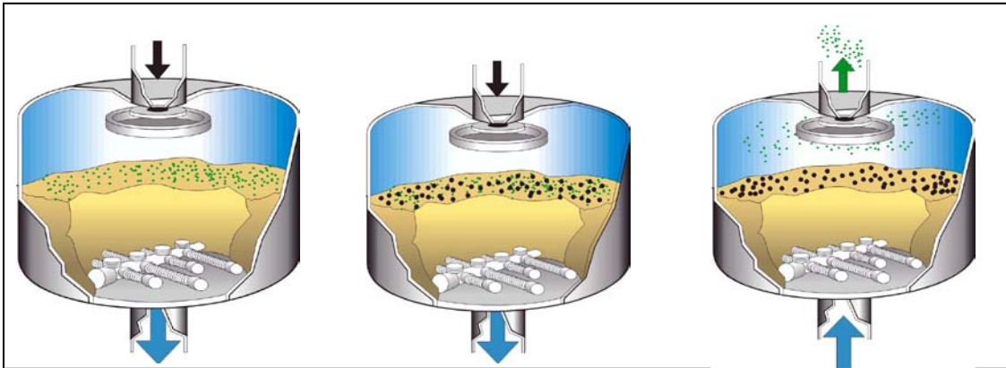
Fine sand & organics (far left) are easily captured by the sand media. Larger/heavier particle matter (middle) also is easily trapped by the sand media. Backwashing, however, has limited influence (far right) on the heavier/larger particle matter, causing residual build-up and greater pressure loss issues.
